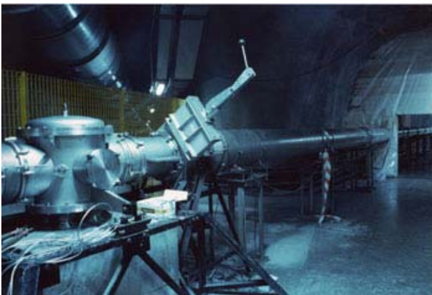
GIGS geodetic interferometers (Credit: INFN)
