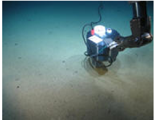
Seismometer connected to the ANTARES secondary junction box (Credit: ANTARES )
