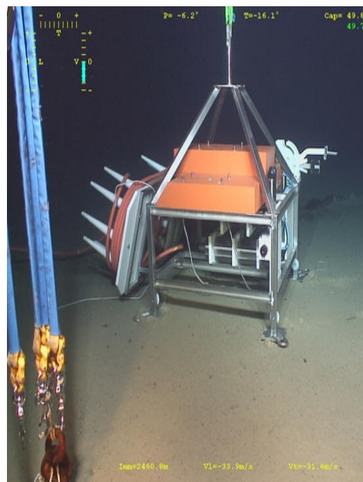
View of the Instrumented Interface Module (MII) that is hosting a CTD sensor, an oxygen sensor, a turbidity sensor, a currentmetre (ADCP) (Credit: ANTARES)
