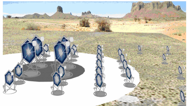
A possible design of CTA. Large mirrors in the centre collect enough light to catch dim showers from low-energy gamma rays. To obtain large statistics at high energies where particles are rare but the associated showers are bright, smaller mirrors cover an area of a few square kilometres (Credit: ASPERA / D. Rouable)
