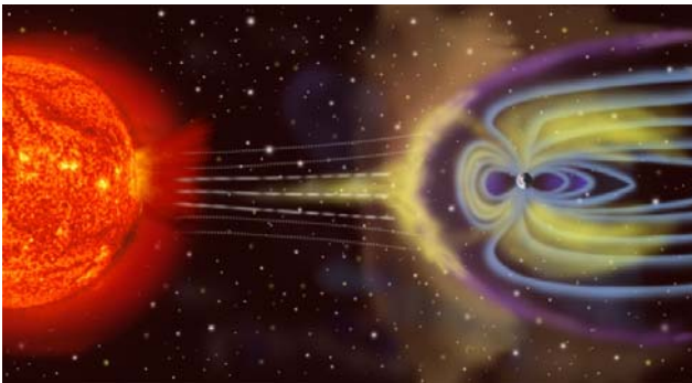
Artist's rendition of Earth's magnetosphere (Credit: NASA).
