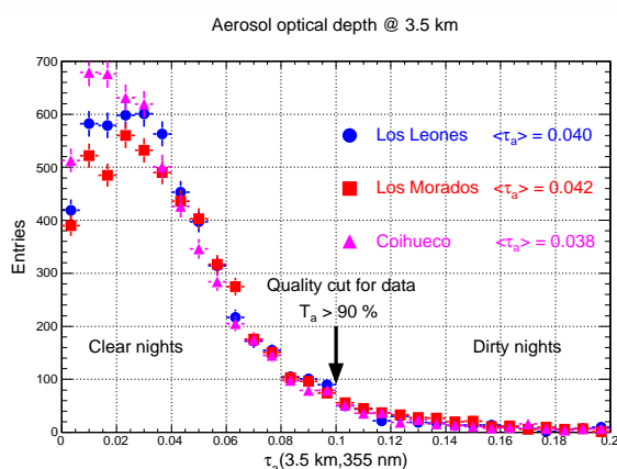
Aerosol measurements. Vertical aerosol optical depth at 3.5 km above the FD measured between January 2004 and December 2010 (from Louedec et al. , 2011).
