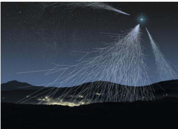
Before reaching the Earth's surface, cosmic ray messengers interact with the constituents of the atmosphere, changing their nature and energy. A large variety of secondary particles, which decay or make new collisions, is produced. (Credit: L.Bret / Novapix / ASPERA)
