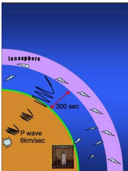
Excitation model: the electromagnetic ionosphere signal arrives BEFORE the seismic ground wave if the epicenter is more than about 2000km away. (Credit: LSBB).
