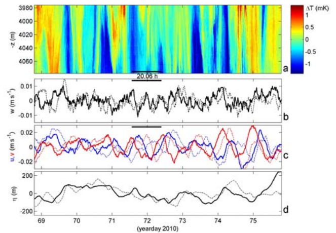
One week of deep internal wave observations. (a) Depth-temperature image relative relative to the adiabatic lapse rate. The inertial period is indicated. (b) Two-hourly smoothed vertical currents observed 2 m above uppermost T-sensor (solid) and 196 m below lowest (dashed). (c) Corresponding horizontal current components u (blue) and v (red). (d) Vertical excursions computed. (Credit: taken from van Haren and Gostiaux (2011)).
