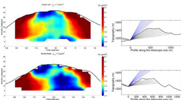
Density profiles obtained on two different views of la Soufrière de Guadeloupe and a sketch of the potential directions of sight (Credit: Jacques Marteau).
