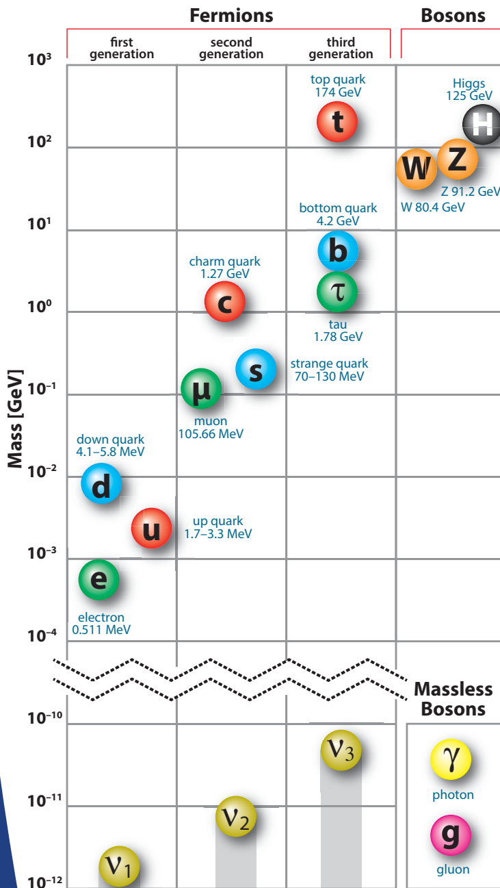
Masses of the particles in the Standard Model. The electron-, muon- and tau-neutrinos are mixtures of the mass-eigenstate neutrinos ( \nu_1 , \nu_2 and \nu_3 ) shown in the illustration.
