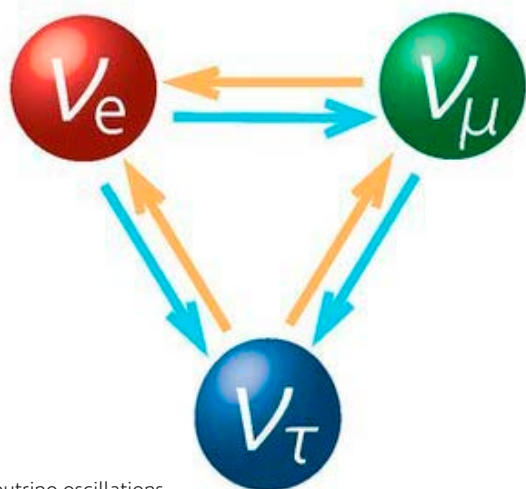
Neutrino oscillations
