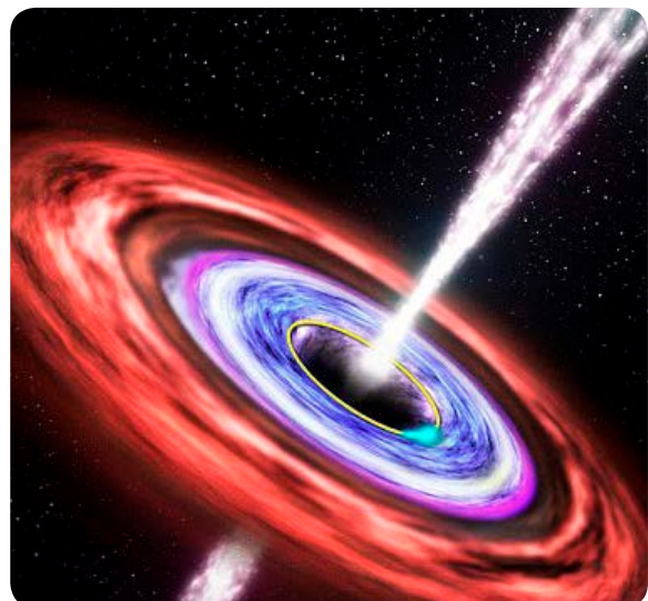
Gamma ray burst schematic
