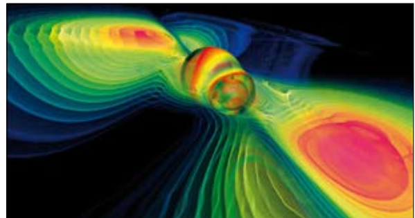
Modelling of gravitational waves produced by the merging of two black holes.
