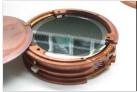
A combination of heat and electrical current in germanium crystals is recorded by the Edelweiss detector in the Laboratoire Souterrain de Modane (France).
