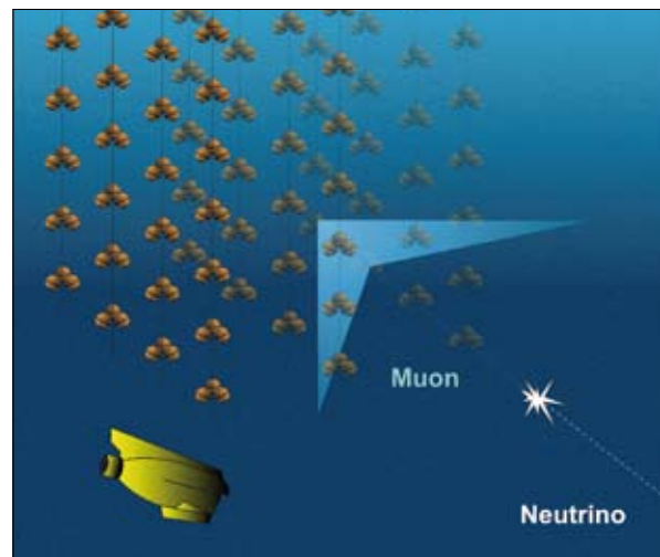
A muon is generated in a neutrino interaction and emits a cone of bluish Cherenkov light. The light is recorded by sensors in pressure tight glass spheres.
