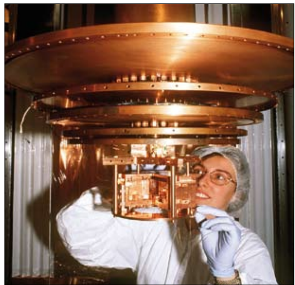
The CRESST detector in the Gran Sasso Laboratory searches for a combination of light and heat signals in crystals cooled down to about 20 milli-Kelvin.
