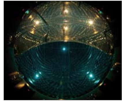
View into the BOREXINO detector being filled with 100 tons of ultra-pure scintillator.
