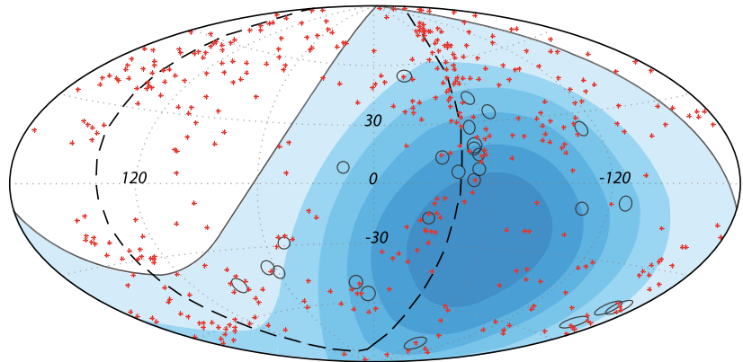
Sky-map of the published 27 highest-energy Auger events (black circles), compared to positions of active galactic nuclei (red crosses).
