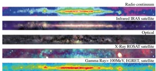
The galactic plane as seen in different wavelengths.
