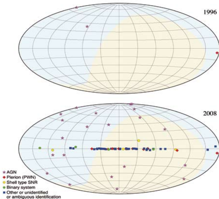
The high energy gamma ray sky, 1996 and 2008
