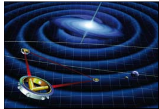
Measuring ripples in space with LISA.
