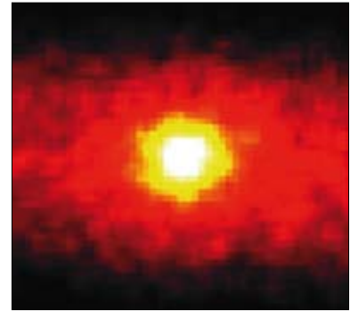
The Sun as seen in neutrinos. The picture is composed from several thousand neutrinos recorded by the Japanese Super-Kamiokande detector.
