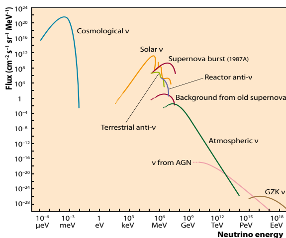
A synoptic view of neutrino fluxes.
